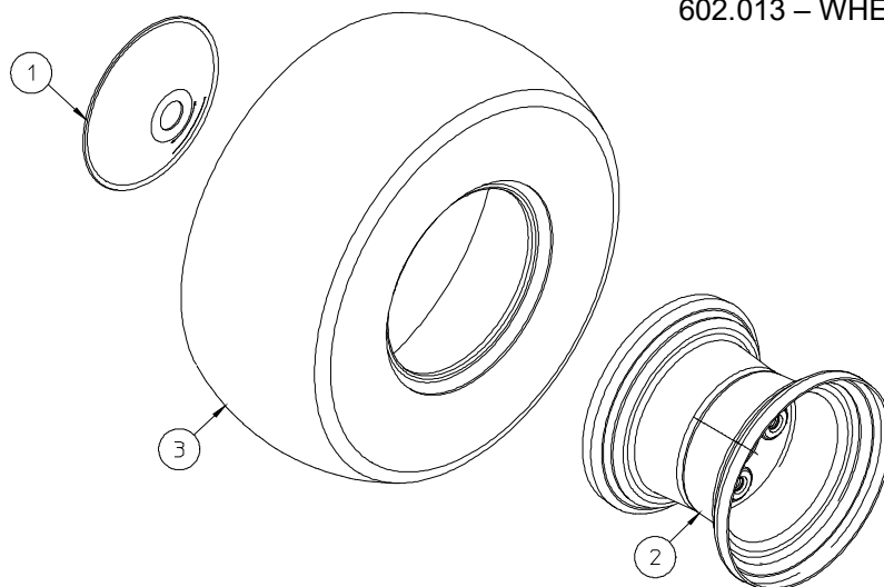
602.013 – WHEEL 18X8.50-8
