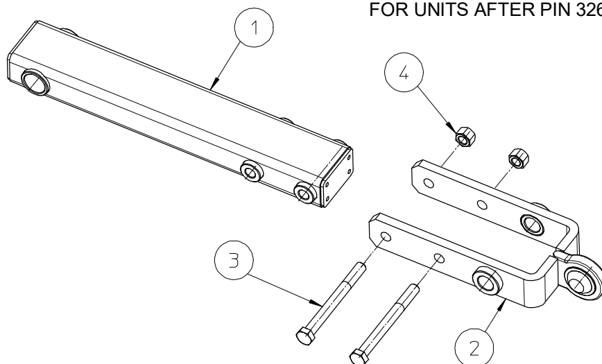
LOWER ARM 270.336 FOR UNITS AFTER PIN 326900
