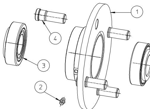
IDLER HUB 270.275
