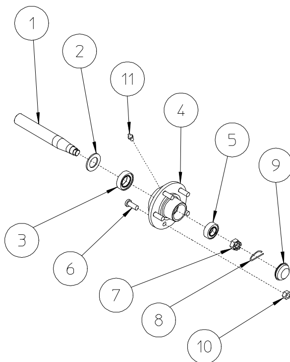
TANDEM HUB 215.960
