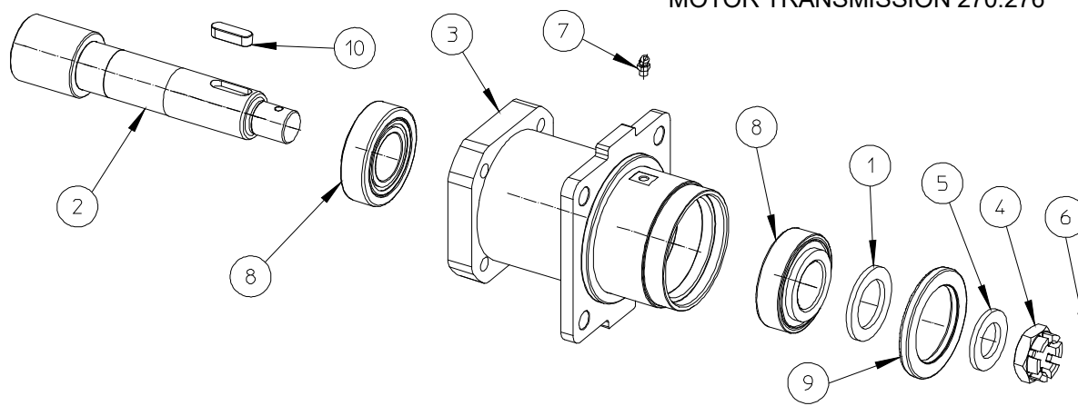
MOTOR TRANSMISSION 270.276
