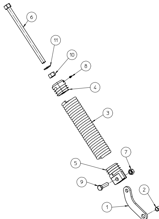
FLOATING SPRING 270.341 FOR UNITS AFTER PIN 326900
