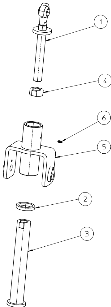
FLOATING LINK 270.358 FOR UNITS AFTER PIN 326900
