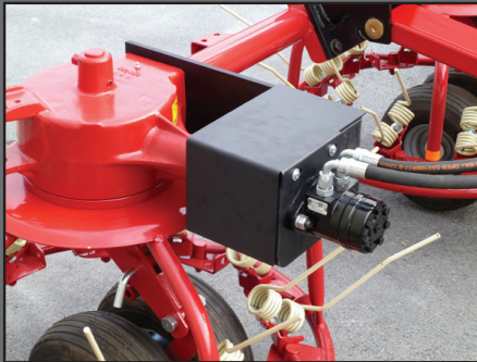
DT-SIT MOUNTING
