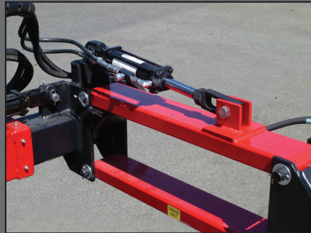
PARALLEL LINKAGE
